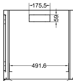
SECTION PLANE A-A
